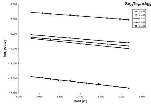
Fig. 1. Temperature dependence of dark conductivity for various samples in amorphous \text{Se}_{70}\text{Te}_{30-x}\text{Ag}_x thin films.
