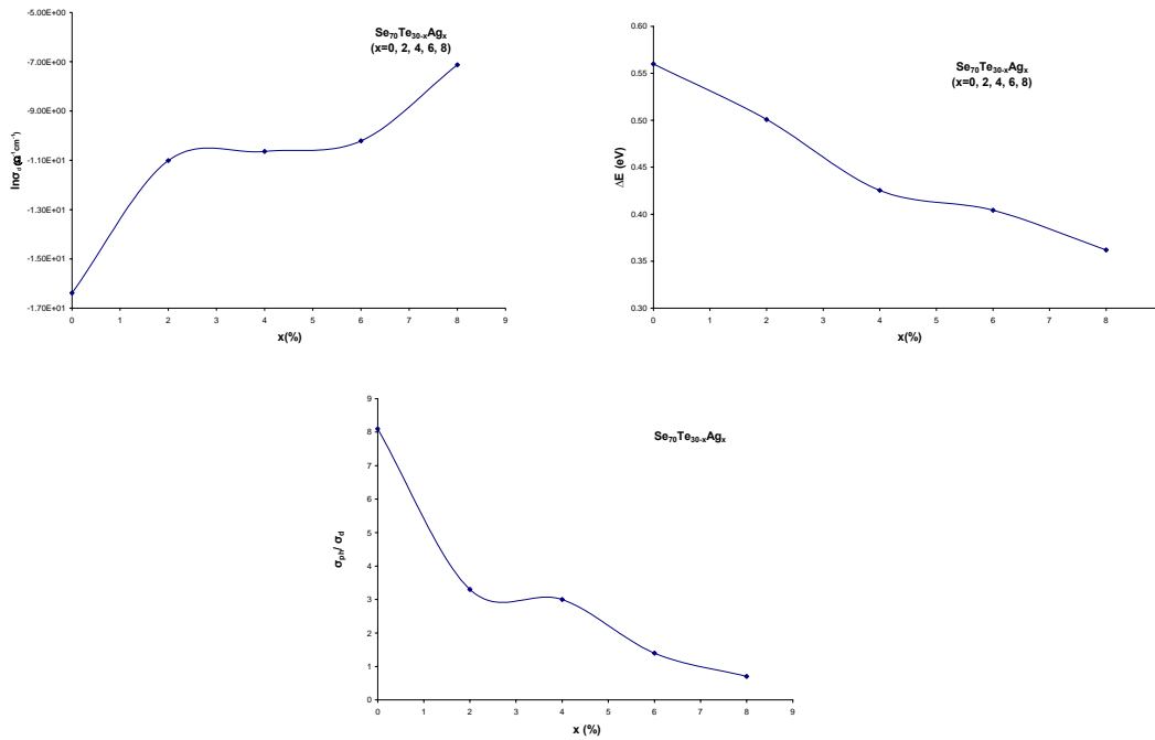
Fig.2. Composition dependence of dark conductivity ( \sigma_d ), activation energy ( \Delta E ) and photosensitivity ( \sigma_{ph}/\sigma_d ) in amorphous Se_{70}Te_{30-x}Ag_x thin films.
