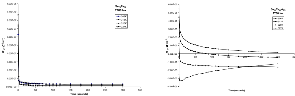
Fig. 6. Decay of photoconductivity at different temperatures in amorphous Se_{70}Te_{30} and Se_{70}Te_{28}Ag_2 thin films
