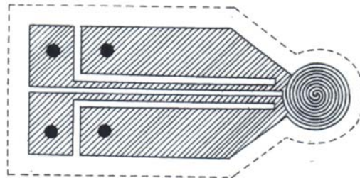
Fig. 1. Schematic diagram of TPS sensor.
