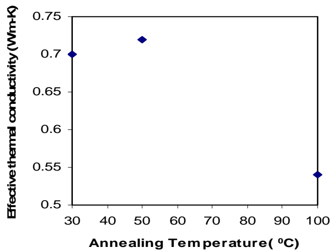
Fig.5. Variation of effective thermal conductivity with annealing temperatures of \text{Se}_{90}\text{In}_{10} chalcogenide glass.
